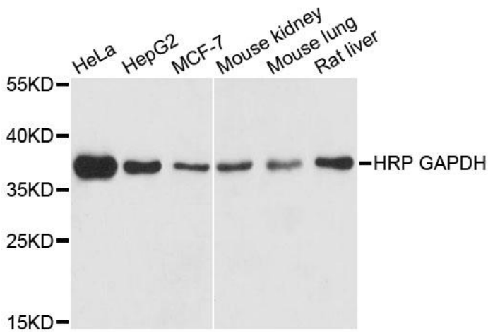
Western blot analysis of extracts of various cell lines, using- HRP-Conjugated GAPDH Antibody at 1:5000 dilution. Lysates/Proteins: 25ug per lane. Blocking buffer: 3% nonfat dry milk in TBST. Detection: ECL Basic. Exposure time: 90s
