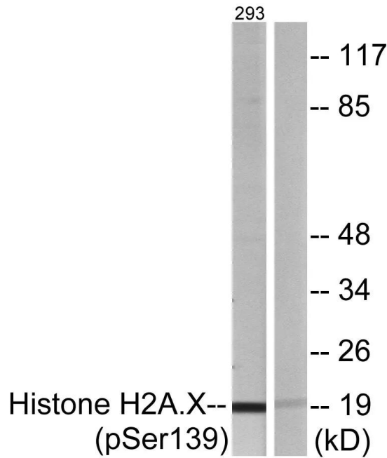
Western blot analysis of lysates from 293 cells treated with heat shock, using Histone H2A.X (Phospho-Ser139) Antibody. The lane on the right is blocked with the phospho peptide.
