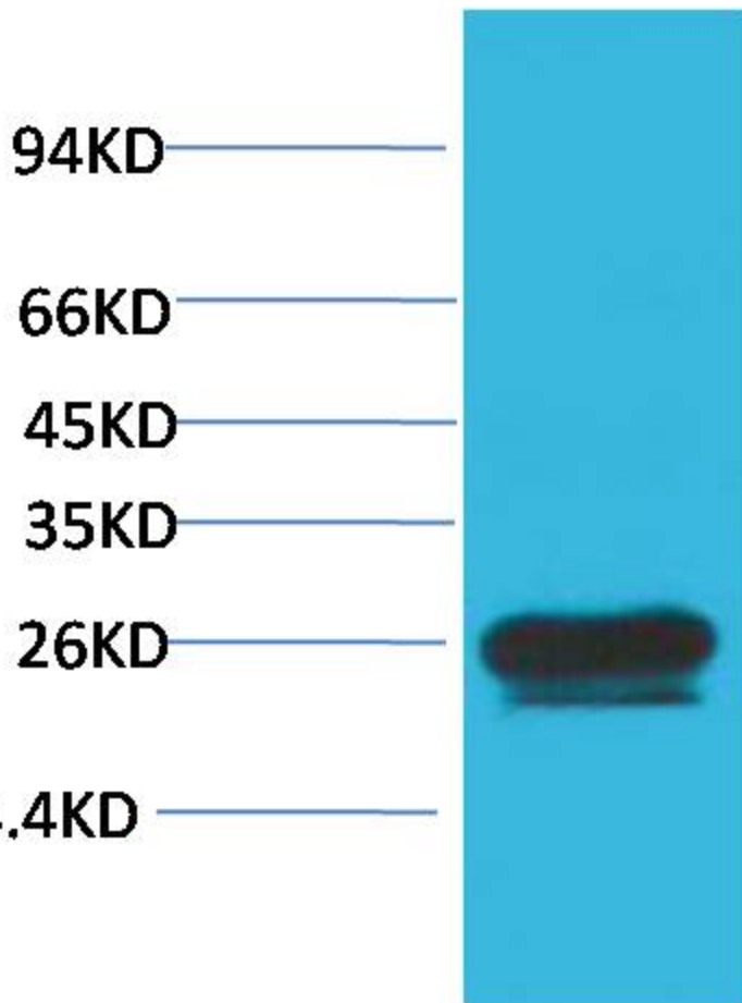
Western blot analysis of Hela with HSP27 Mouse mAb diluted at 1:2,000.
