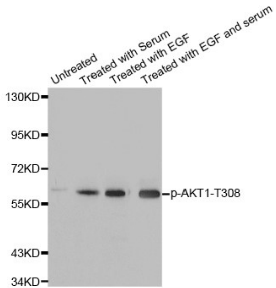
Western blot analysis of extracts from HeLa cells using Phospho-AKT1-T308 antibody (ABP-0304). Secondary antibody: HRP Goat Anti- Rabbit IgG (H+L) at 1:10000 dilution. Lysates/proteins: 25ug per lane. Blocking buffer: 3% BSA.
